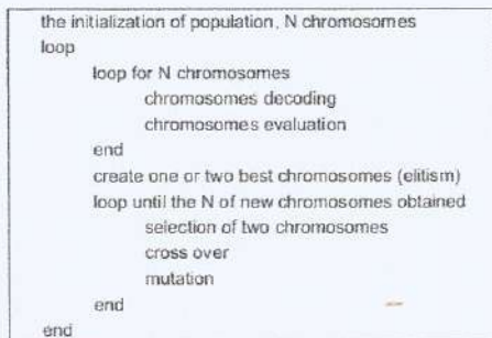
Fig.2. Pseudocode of genetic algorithm method
