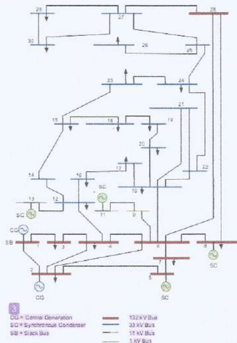
Fig. 4. The IEEE 30 bus test system
